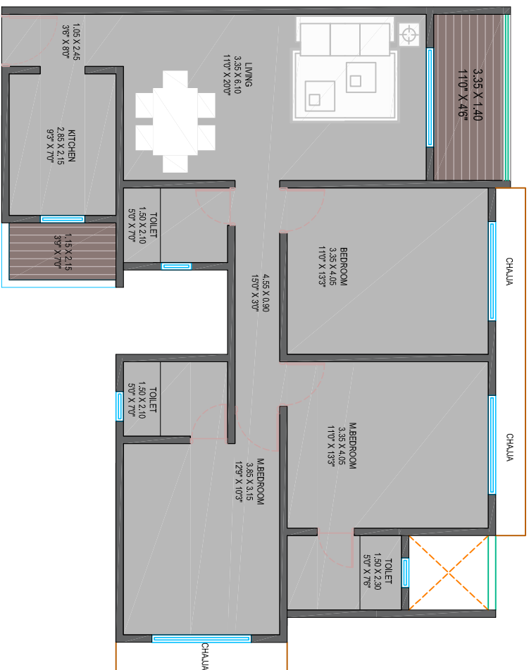
CARPET AREA 90.83 SQ.MT 977.69 SQ.FT
