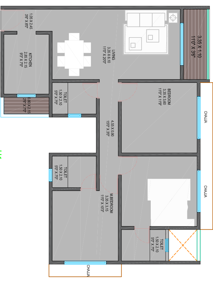
CARPET AREA 84.40 SQ.MT 908.48 SQ.FT (E)
